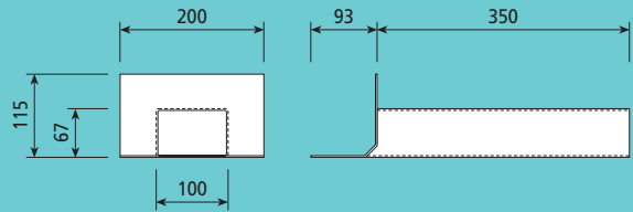
BT 301 Scupper
