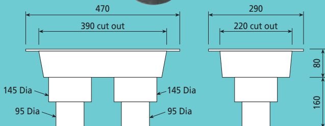
BT 205 Rainhead Moulded rainhead with overflow. To suit 100mm or 150mm downpipe.
