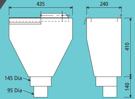
BT 202 External Rainhead Moulded rainhead with metal fixing strip. To suit 100mm or 150mm downpipe. Can be used in conjunction with BT 301 Scupper.
