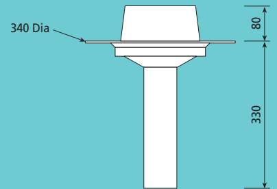
BT 400 Roof Vent
