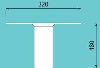
BT 608, BT 609, BT 610 Drain
